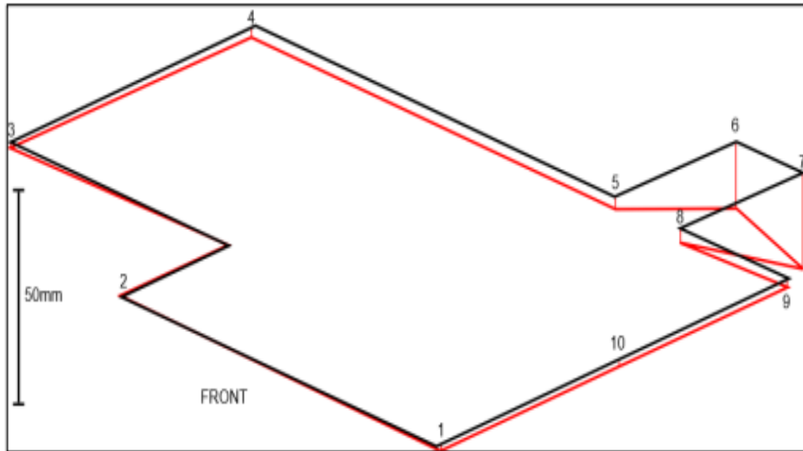
Figure 4. Isometric sketch showing the amplitude of movements at each monitoring location. The focus of movement is at markers 6 and 7 at the rear of the conservatory.
